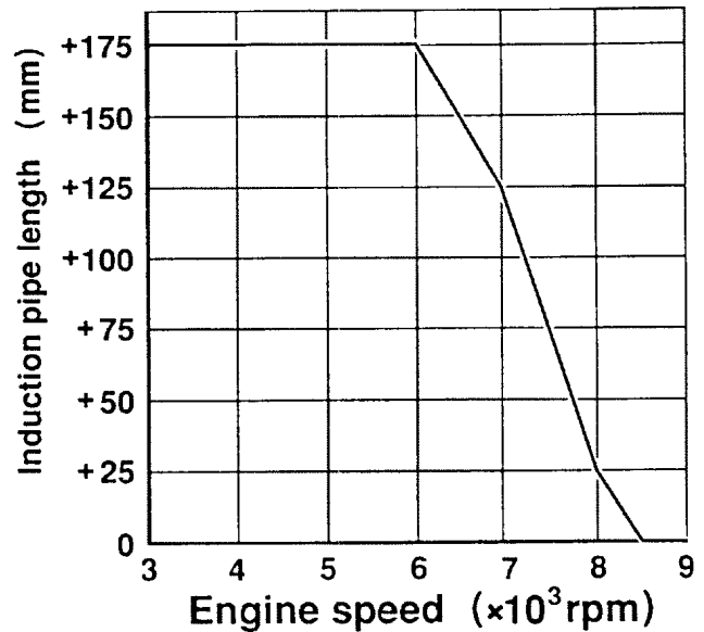
Fig. 11 Induction pipe length vs engine speed
