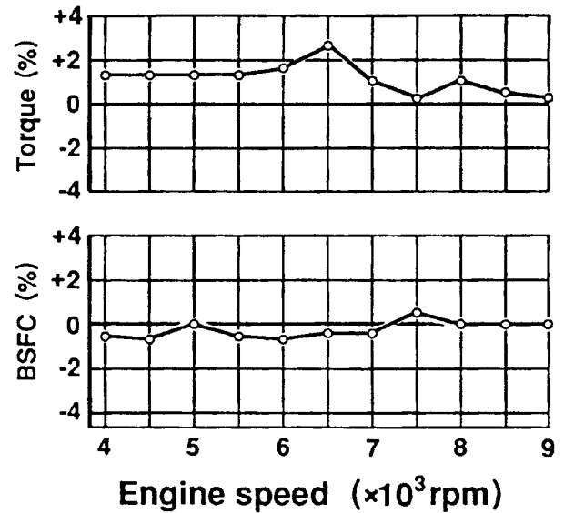
Fig. 20 Effect of 2-piece apex seal on output and BSFC (Comparison with one-piece apex seal)
