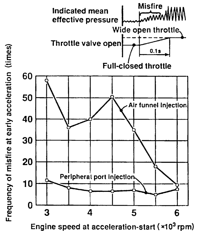
Fig. 15 Response at steep acceleration
