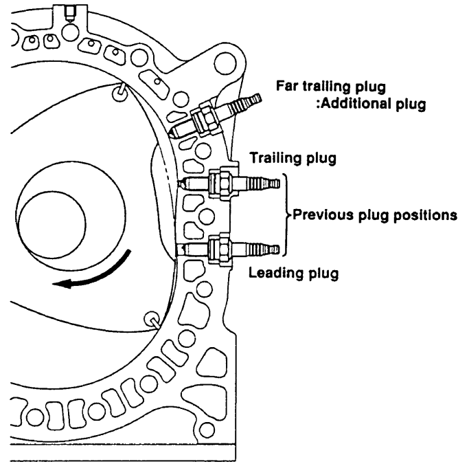
Fig. 17 3-plug ignition system
