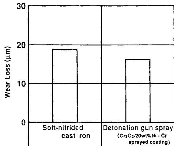
Fig. 23 Result of reciprocating wear rig tests
