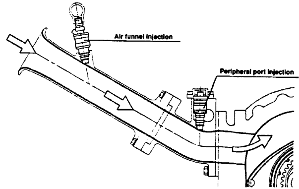
Fig. 14 Peripheral port injection & air funnel injection
