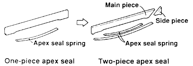
Fig. 19 Modification of apex seal
