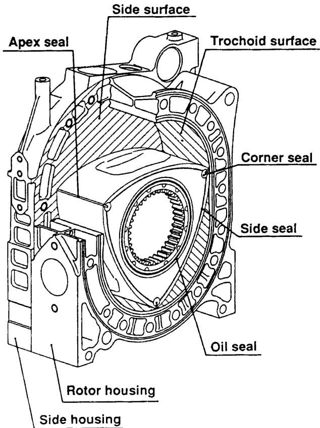
Fig. 21 Cermet coating (Shaded area)
