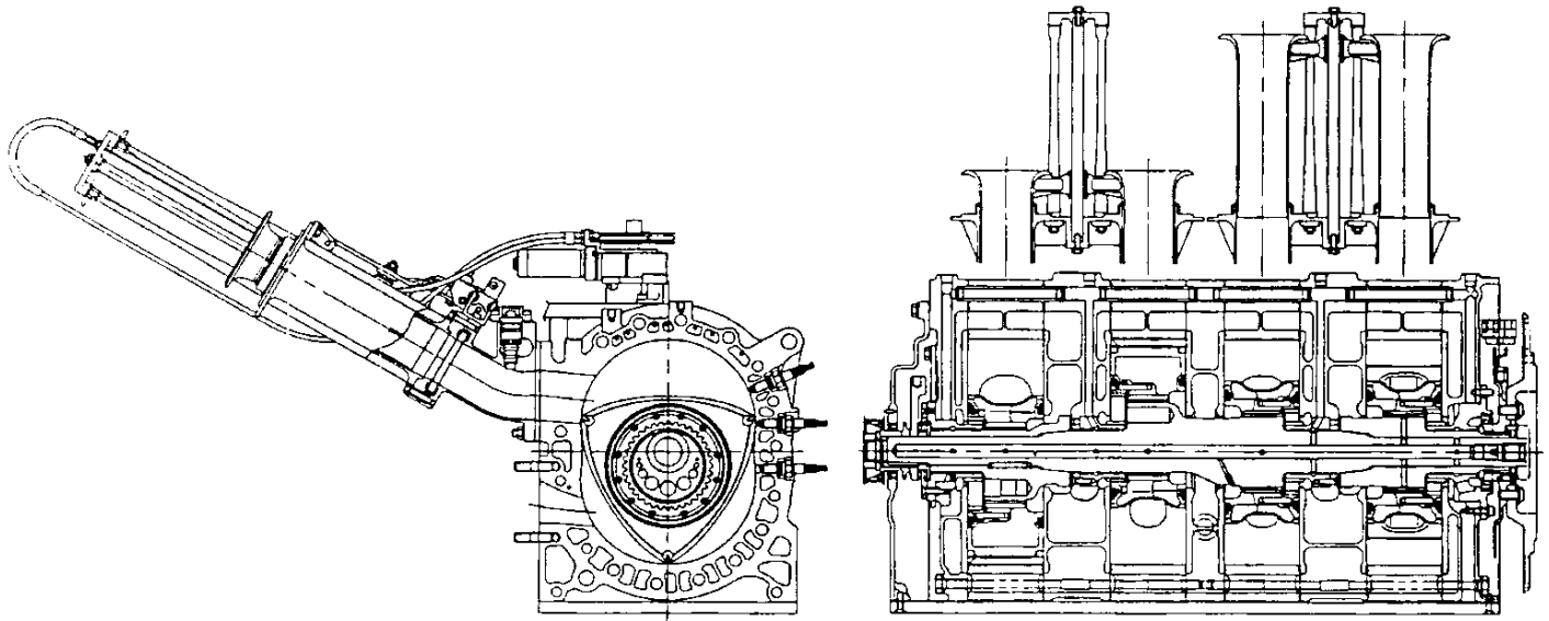
Fig. 4 Sectional view of R26B
