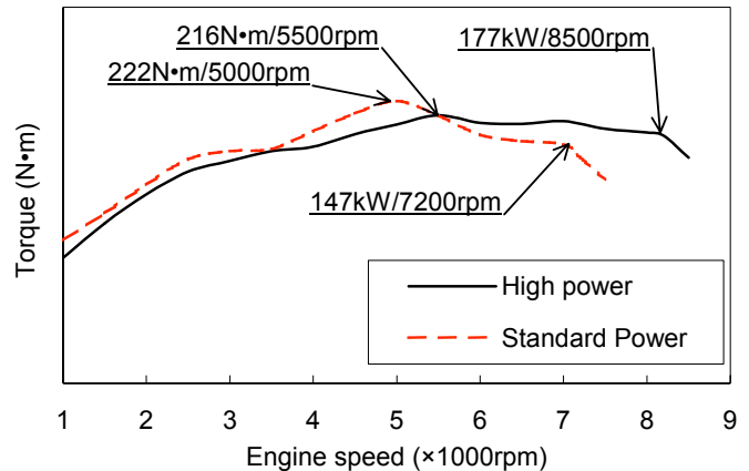
Fig.3: Engine Output Performance
