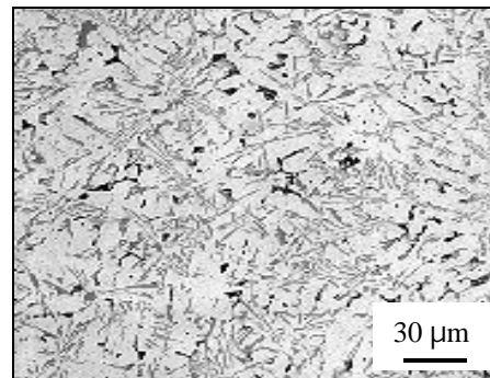
MSFC-388 typical microstructure (Eutectic alloy)
