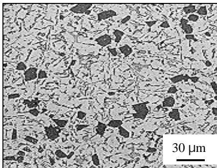
MSFC-398 typical microstructure (Hypereutectic alloy)
